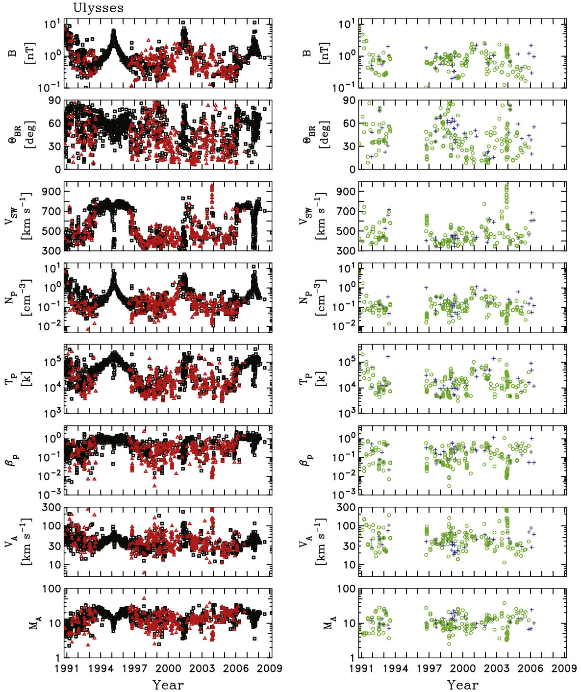
Figure 2. Ambient plasma parameters for the times studied here. (left column) Wave and control intervals are again represented by red triangles and black squares, respectively. (top to bottom) We plot the average magnetic field intensity B in nT, the angle between the mean field and the radial direction \Theta_{BR} in degrees, the mean solar wind speed V_{SW} in units of \text{km s}^{-1} , the thermal proton density N_P in units of \text{cm}^{-3} , the thermal proton density T_P in units of Kelvin, the proton energy density parameter \beta_p , the Alfvén speed V_A in units of \text{km s}^{-1} , and the Alfvén Mach number M_A . (right column) Same for wave intervals with |E_{lip}| \geq 0.35 (green circles) and intervals showing evidence of possible \text{H}^+ acceleration (blue pluses).
